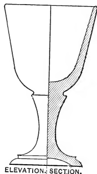
ELEVATION, SECTION.
